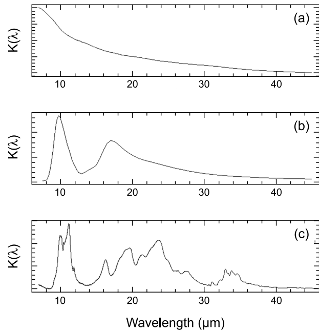
Fig. 3. Mass absorption coefficient (in arbitrary units) of (a) amorphous C, (b) amorphous olivine, and (c) crystalline olivine (Bruzato et al. , 1999b).
