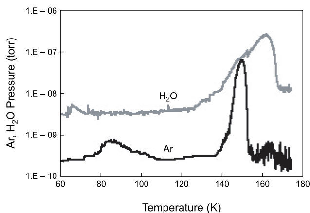
Fig. 5. Gas evolution from a 0.1- \mu\text{m} amorphous gas-laden ice sample upon its warming up. The gas comes out when the amorphous ice transforms into its crystalline and “restrained amorphous” forms.
