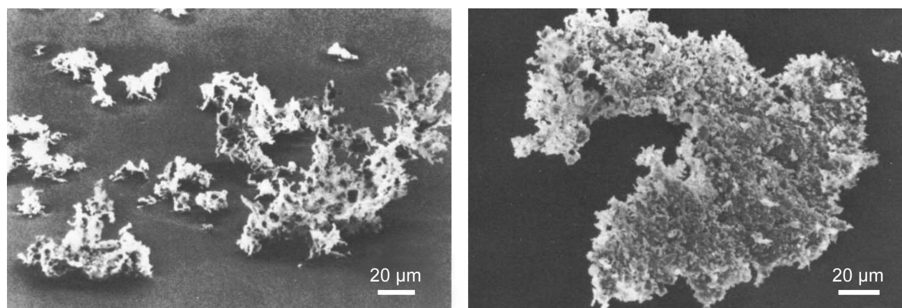
Fig. 7. SEM micrographs of dust grains emitted during the KOSI-3 experiment.
