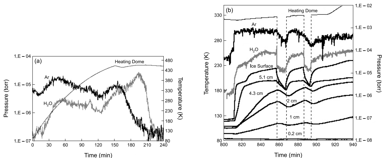
Fig. 9. (a) Evolution of Ar trapped in the ice and ice sublimation, upon heating from above of a 0.5\text{-cm} -thick sample. Note the early rise of the Ar and its exhaustion before all the ice sublimates. (b) Temperature profiles of the thermocouples as a function of their distance from the 80\text{-K} bottom plate in a 6\text{-cm} -thick ice deposit. Note also the sharp decrease and increase of the water flux vs. the sluggish response of the Ar emanation, when the ice sample is covered by the cold plate and upon its removal.
